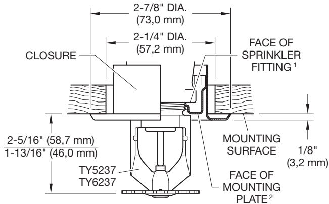
FIGURE 1 SERIES EC-11 TY5237 AND EC-14 TY6237 PENDENT SPRINKLER ASSEMBLY WITH 3/4 INCH TOTAL ADJUSTMENT STYLE 60 TWO-PIECE FLUSH ESCUTCHEON
