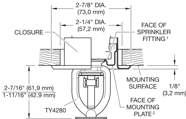
FIGURE 4 SERIES TY-L TY4280 8.0K STAINLESS STEEL PENDENT SPRINKLER ASSEMBLY WITH STYLE 60 TWO-PIECE FLUSH ESCUTCHEON
